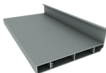
Bottom Base Profile Product Code: 37266 Weight kg/m: 1,483 (15 x 127 x 43 x 1,5mm)
