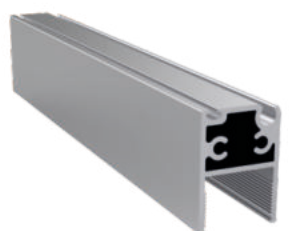
22mm Railing Profile Product Code: 3067 Weight kg/m: 0,800 (38,7 x 27 x 1,7mm)
