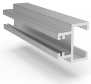
Rail Upper Add Product Code: 2421 Weight kg/m: 1,171 (43 x 40 x 3mm)
