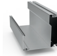
Common Gutter Adapter Product Code: 6536 Weight kg/m: 2,618 (39 x 100 x 4mm)
