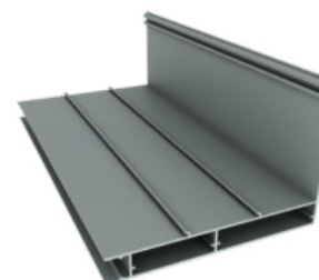
8mm Adapter Profile Product Code: 37281 Weight kg/m: 0,353 (24,6 x 16,1 x 1,25mm)
