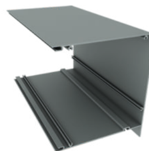
22mm Post & Bottom Profile Product Code: 37263 Weight kg/m: 0,545 (28 x 35 x 1,6mm)
