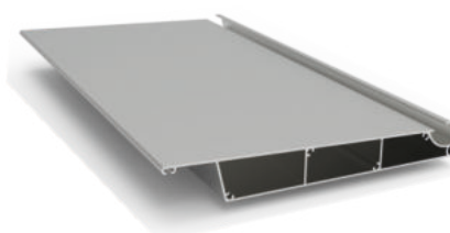
Lamella Product Code: 2340 Weight kg/m: 3,906 (40 x 286 x 2 mm)
