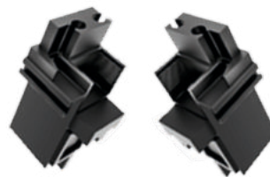
Fixed Corner Wedge Top Product Code: LTS-8 Qty in One Set: 2 Pcs
