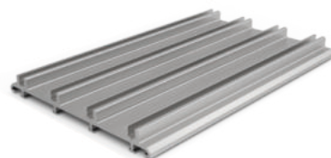
Bottom Case Profile Product Code: 2070 Weight kg/m: 1,480 (15,5 x 130 x 2mm)
