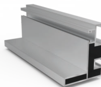
Rail Product Code: 2422 Weight kg/m: 3,933 (110 x 94 x 3mm)
