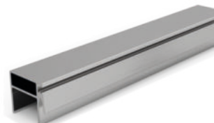
Side Case Profile Cover Product Code: 2067 Weight kg/m: 0,186 (13,6 x 27 x 1,3mm)
