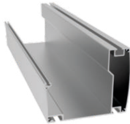
Standard Gutter Product Code: 5935 Weight kg/m: 3,916 (158 x 125 x 2,5mm)
