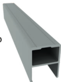
Rail Cover Profile Product Code: 37270 Weight kg/m: 0,230 (13 x 39 x 1,3mm)
