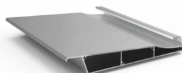
Lamella Product Code: 2420 Weight kg/m: 3,700 (274 x 40 x 2mm)
