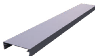
Top Cover Profile Product Code: 2535 Weight kg/m: 0,312 (16 x 62 x 1mm)
