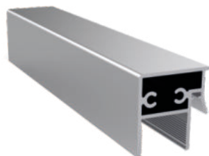
22mm Puller Profile Product Code: 3068 Weight kg/m: 0,860 (38,7 x 35,25 x 1,5mm)
