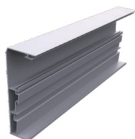
Wall Connection Profile Product Code: 2532 Weight kg/m: 2,651 (191 x 69 x 1,8mm)
