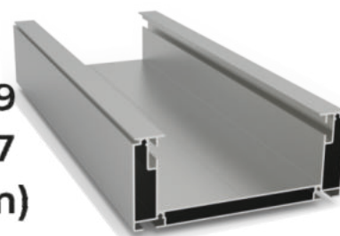
Gutter Product Code: 2337 Weight kg/m: 4,560 (85 x 205 x 2 mm)
