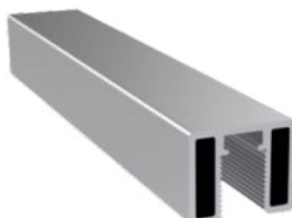
8mm Adapter Profile Product Code: 3065 Weight kg/m: 0,370 (18,25 x 22,2 x 1,4mm)
