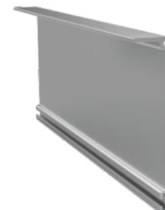
Internal Nail Profile Product Code: 3073 Weight kg/m: 0,540 (78,2 x 18,23 x 1,8mm)
