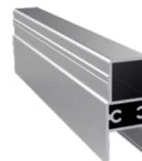
22mm Mid-Panel Side Post Profile Product Code: 3064 Weight kg/m: 1,030 (57,5 x 27 x 1,7mm)
