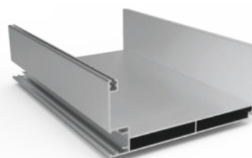
Gutter Product Code: 2423 Weight kg/m: 3,512 (199 x 86 x 2,5mm)
